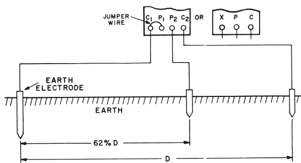
Fig. 11: Fall-of-potential or three-terminal earth resistance test
