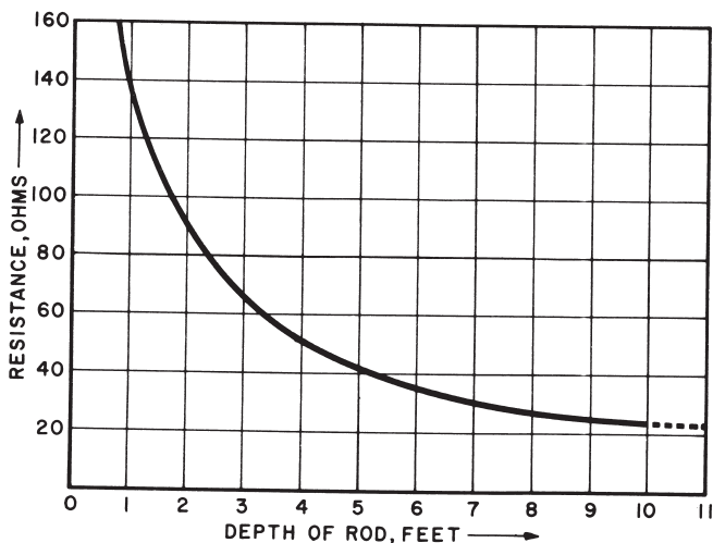
Fig. 15: Earth resistance decreases with depth of electrode in earth (Source: Ref 19)
