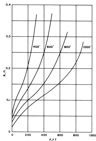
Fig. 29: Earth resistance curves for a substation
