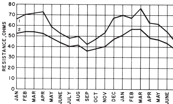
Fig. 4: Seasonal variation of earth resistance with an electrode of 3/4" pipe in stony clay soil. Depth of electrode in earth is 3 ft for Curve 1 and 10 ft for Curve 2 (source: Ref. 9, page 76)
