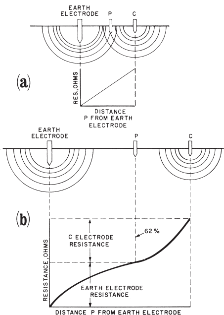
Fig. 13: Effect of C location on the earth resistance curve
