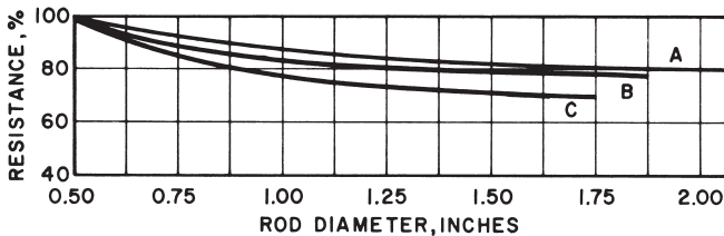
Fig. 16: Diameter of a rod has little effect on its earth resistance
