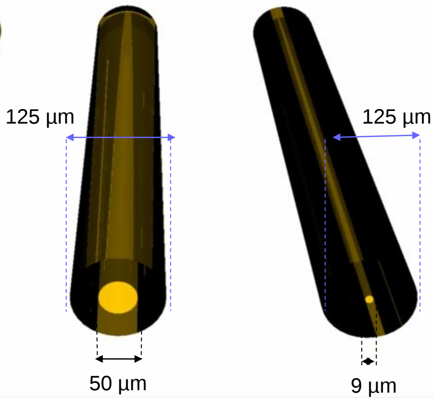
Singlemod-fiber
