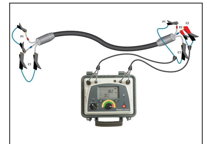
Fig 13: The other end of the cable shows the unmarked core carrying C1 connected to core with the blue marker (the core to be tested) and the core with the red marker carrying P1 connected to core with the blue marker (the core to be tested) the connections with short jumper cables
