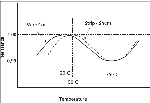
Fig 1: Qualitative Resistance Temperature Curve for Manganin iii
