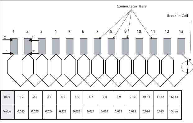
Fig 34: Wave winding test data
