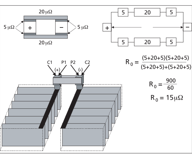
Fig 36: Single strap resistance target
