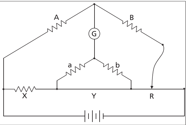
Fig 39: Kelvin bridge circuit viii
