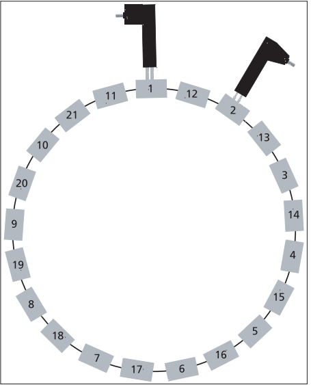
Fig 35: Wave winding coil arrangement
