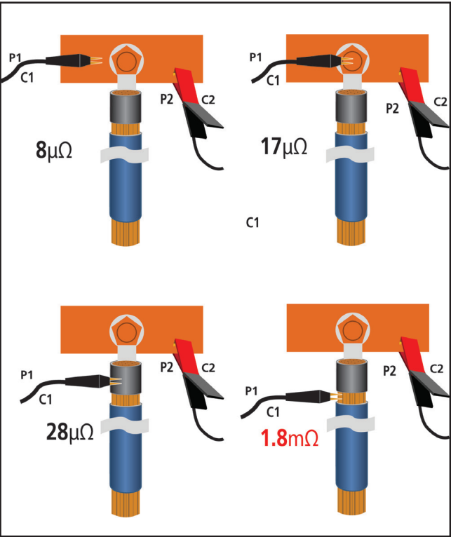
Fig 24: Duplex hand spike being used to perform same test as shown in Fig 23
