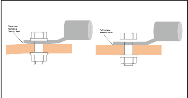
Fig 14: Contact area reduced due to overtightening
