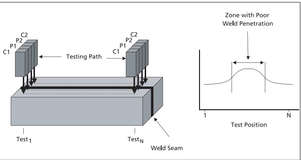
Fig 7: Series of measurements across a weld seam
