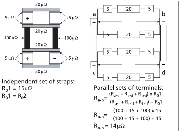
Fig 37: Parallel strap resistance target
