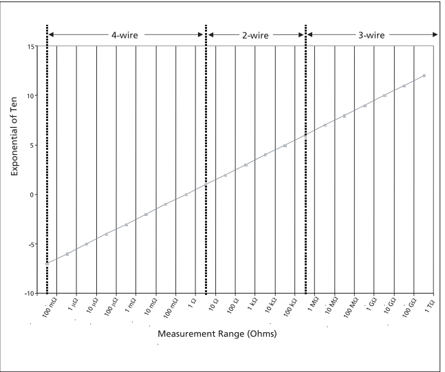
Fig 17: Selection of optimum measuring technique
